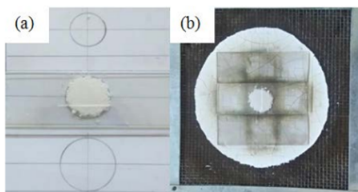
Figure 1. Top view pictures of the SnCl 2 powder and glass slides arrangements. (a) The SnCl 2 powder (white color) arranged in a circular form with a diameter of 1 cm, and (b) the glass slides arrangements with the sandwiched SnCl 2 in the middle and two other glass slides on its left and right sides
